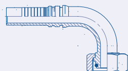
Interlock 90° Swept Female Metric Heavy Serie 24° Cone Seat Swivel (DKOS 90) 26.5193
