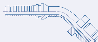
SAE Inverted 45° Flare 45° Elbow Male 23.2240
