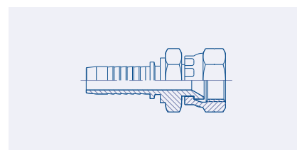
Female JIS 60° Cone Seat Swivel (TOYOTA) 23.3712
