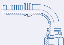
90° Swept Female SAE 45° Swivel 23.4S92
