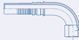
Interlock 90° Swept Female ORFS Swivel 26.4494
