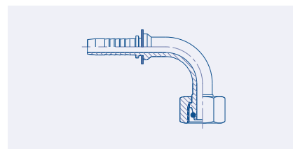
90° Swept Female Metric Heavy Serie 24° Cone Seat Swivel (DKOS 90) 23.5193
