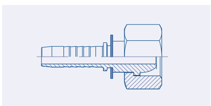
Female Metric 24°/60°C one Seat Swivel (DKL) 23.5213
