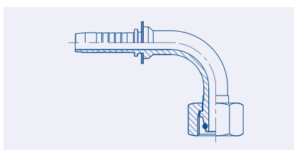
90° Swept Female Metric French Serie 24° Cone Seat Swivel (DKF) 23.5593
