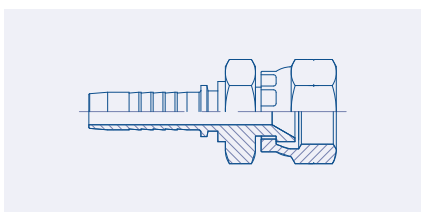
Female JIS 60° Cone Seat Swivel (KOMATSU) 23.5911
