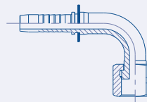
90° Swept Female ORFS Swivel 23.4494
