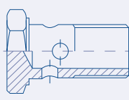
Metric Banjo Bolt 88.1650
