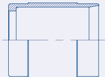
NON SKIVE Balfit® PTFE Convoluted Ferrule 20.TFC
