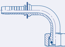
90° Swept Female Metric Heavy Serie 24° Cone Seat Swivel (DKOL 90) 23.5093
